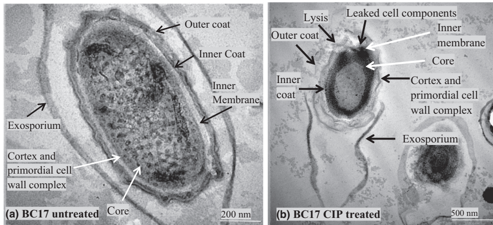
Figure 3 Transmission electron microscopy (TEM) images of B. cereus spores from strain BC17 isolated from filler nozzles of extended shelf life (ESL) milk processing lines showing (a) untreated intact spore and (b) damage to the spore layers following simulated cleaning in place (CIP) treatment.
