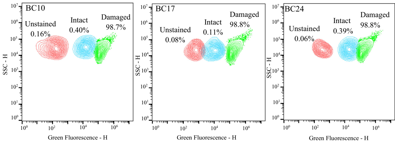
Figure 1 Flow cytometry (FCM)-derived contour plots of side scatter (SSC) versus green fluorescence intensities emitted by SYTO 9-stained intact and damaged B. cereus spores following simulated cleaning in place (CIP) treatment.
